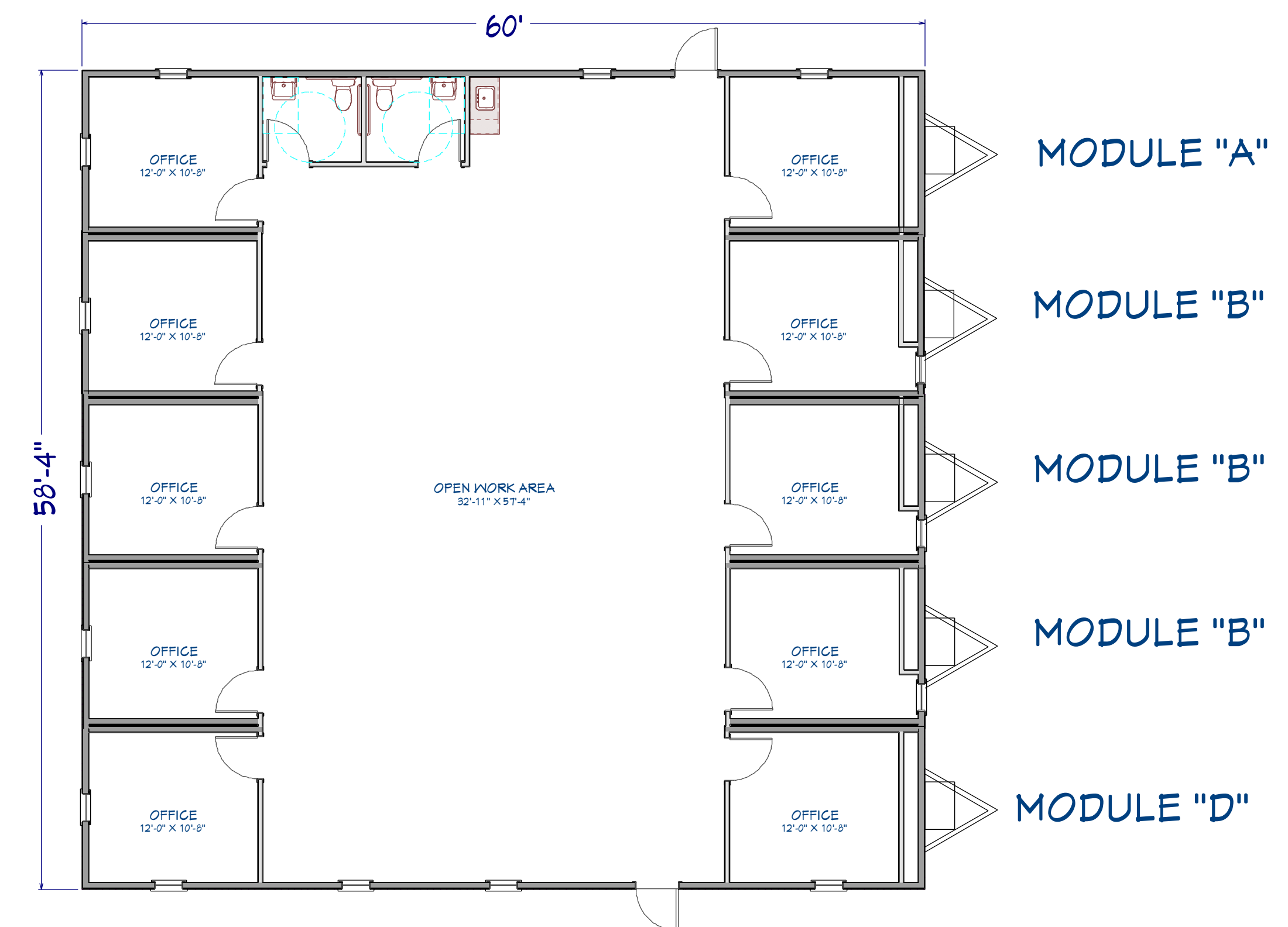
EXAMPLE OFFICE 4 - 60X60 USING MODULES A, B, B, B & D
