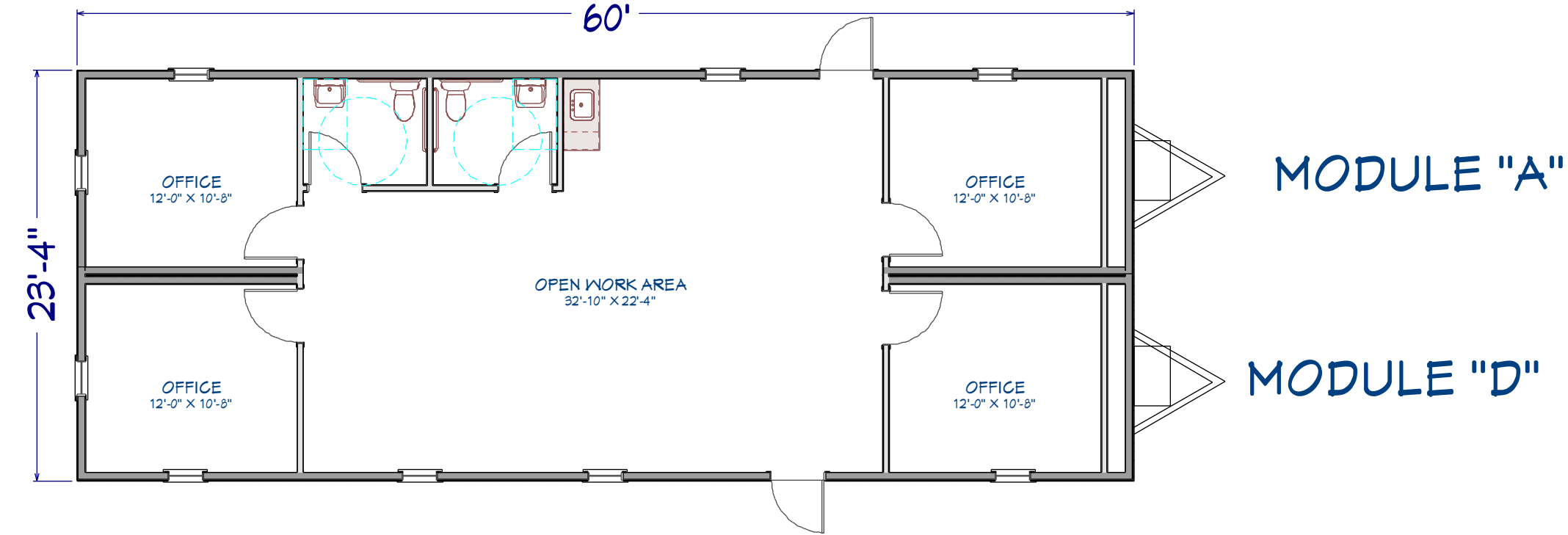
EXAMPLE OFFICE 1 - 24X60 USING MODULES A & D
