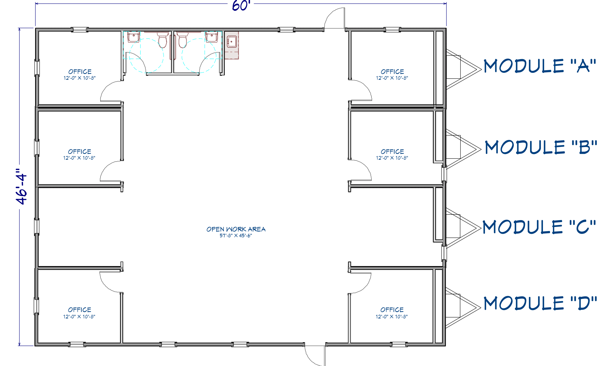
EXAMPLE OFFICE 3 - 47X60 USING MODULES A-D
