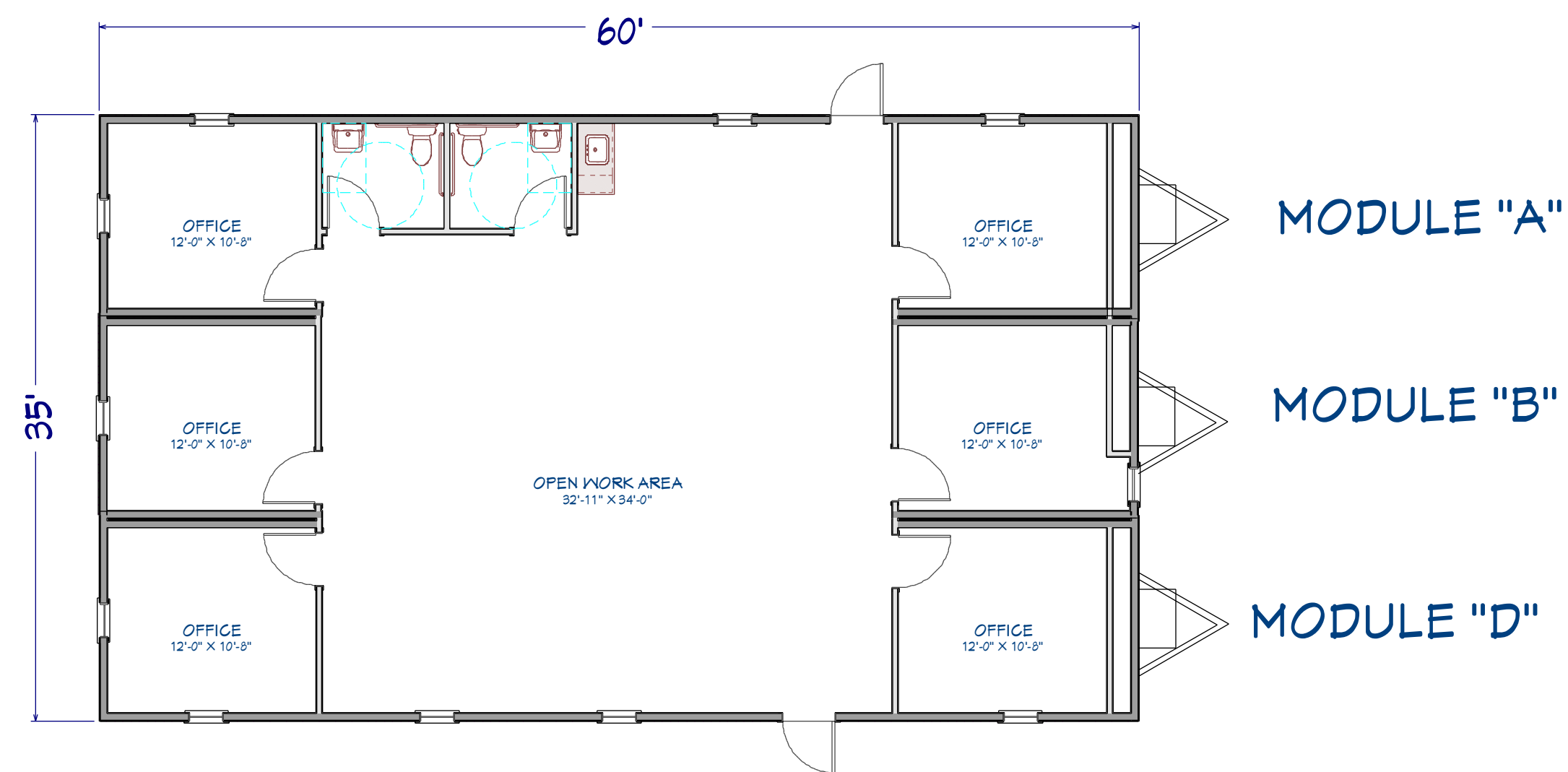
EXAMPLE OFFICE 2 - 35X60 USING MODULES A, B, & D
